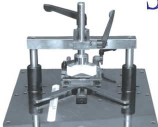
Panel: The top panel is equipped with horrizontal and vertical adjustable clamps for better grip of the mouldings for best joint.
